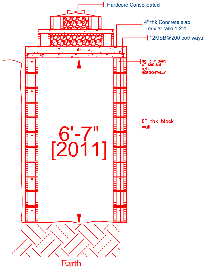
Sectional 1-1
