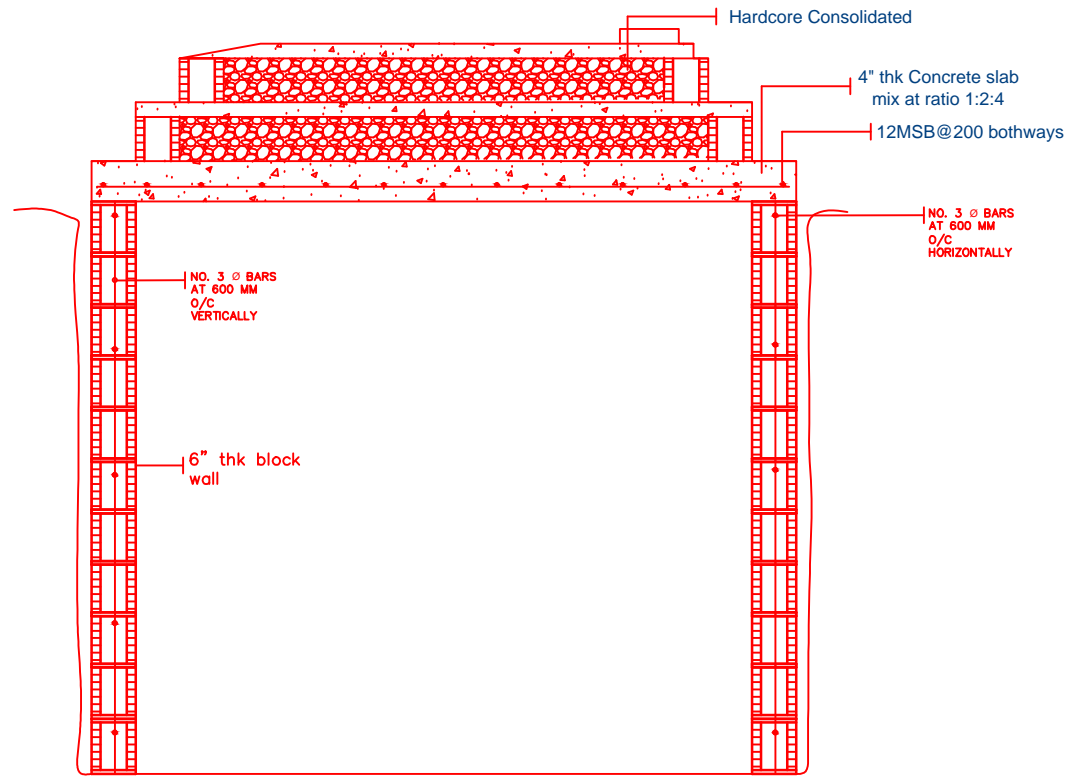
Sectional 2-2
